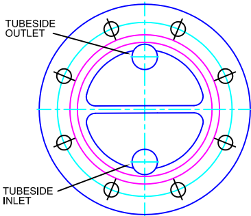
2-PASS DESIGN
