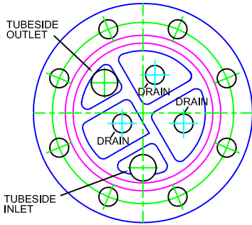
8-PASS DESIGN
