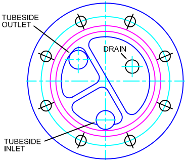
4-PASS DESIGN
