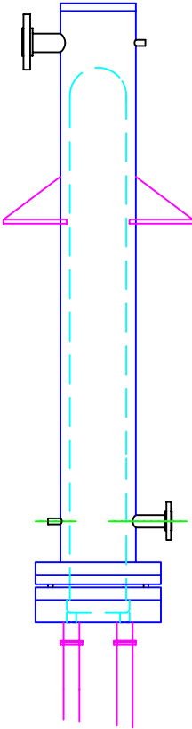
8-PASS DESIGN
