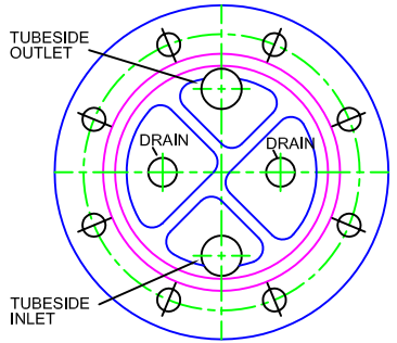
6-PASS DESIGN
